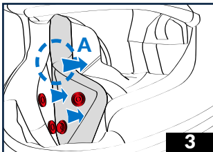
3 - Turn the helmet over again to more easily undo two front snap fasteners, one side velcro fastener and one rear snap fastener on each cheek pad. Hold the two velcro surfaces on either side in place as much as possible in order to gently loosen the area (A).
